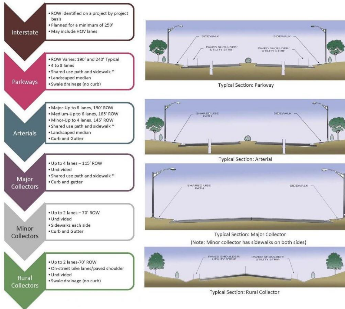
Figure 2 - Typical Standard Section Source: City of Virginia Beach Public Works Design Standards Manual, 2022
