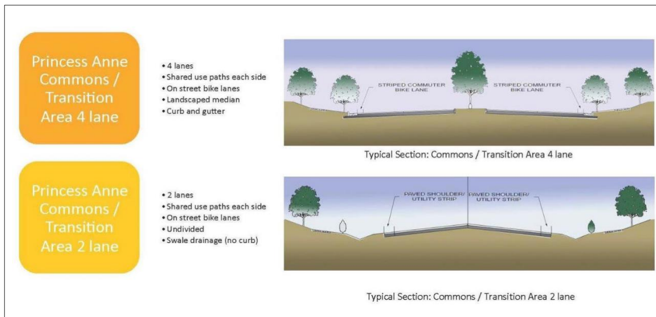
Figure 3 - Typical Section for Princess Anne Commons/Transition Area Roadways Source: City of Virginia Beach Public Works Design Standards Manual, 2022
