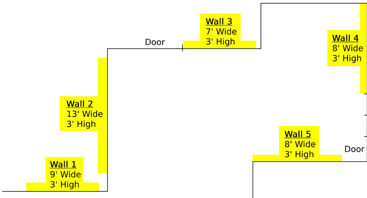
Image 1: Layout of Great Neck Library Art Gallery showing five walls. Wall 1 is 9' wide, Wall 2 is 13', Wall 3 is 7', Wall 4 is 8', Wall 5 is 8'; all 3' high. Doors flank Wall 3 and Wall 5.
