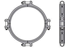
Sizes 20"-24"
