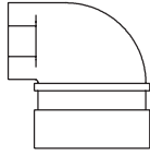
FIG. SE-5 REDUCING 90° ELBOW GROOVE X THREAD
