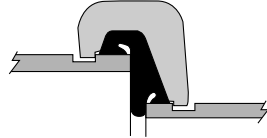
Fig. 7010 Coupling with Gasket
