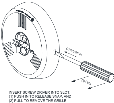
Figure 5: Grille Removal **
