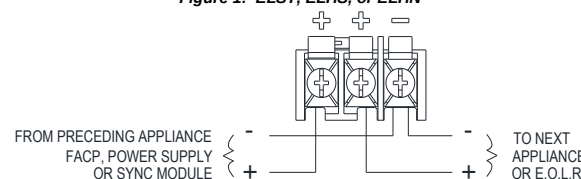
Figure 1: ELST, ELHS, or ELHN
