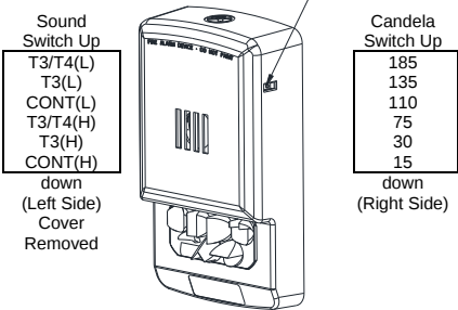
Figure 3: Settings (Set from rear) Factory Setting is 15cd and T3(H). CANDELA
