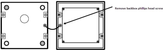
Figure 3. Remove backbox ground wire screw
