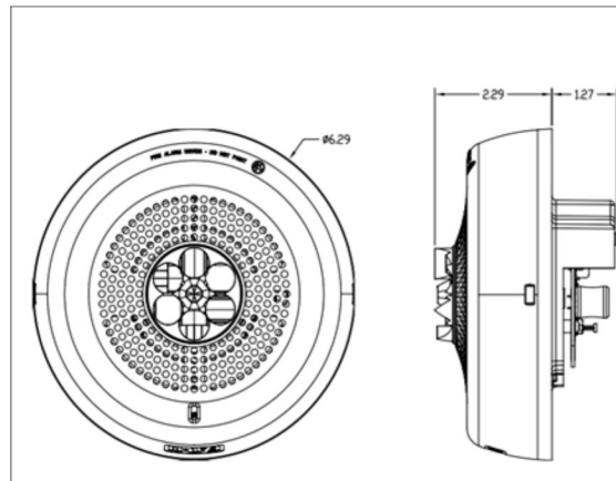
Figure 2. Ceiling multitone strobe
