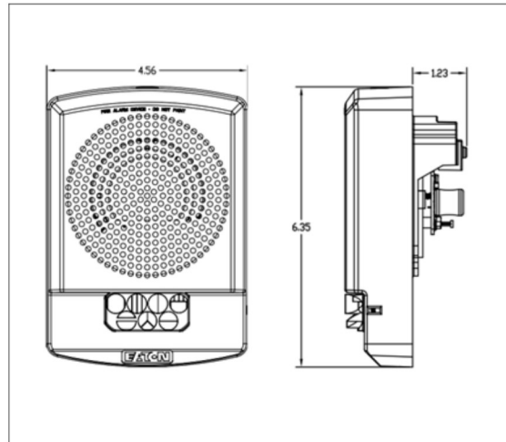
Figure 1. Wall multitone strobe
