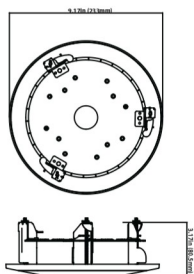
VT-TFMT-L2 In-ceiling Semi-flush Mount
