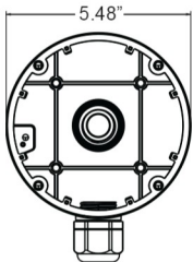
VT-TJB010 Optional Junction box for Cable Management
