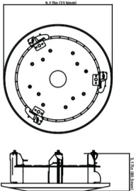
VT-TFMT-L2 In-ceiling Semi-flush Mount
