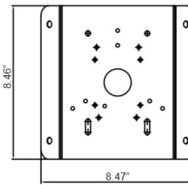
VT-TCNMT Universal Transcendent Corner Mount Adapter
