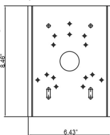
VT-TPLMT Transcendent Universal Pole Mount - Ivory, reqs. VT-TJB08
