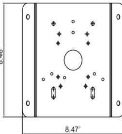
VT-TCNMT Transcendent Universal Corner Mount - Ivory, reqs. VT-TJB08
