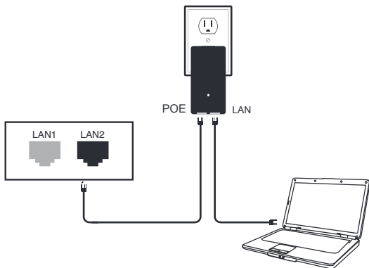
Connecting diagram
