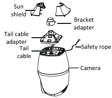
Figure 1 Camera components
