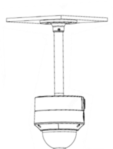
Junction Box: TP-FEJB Pendant Base: TP-AIPMB Extension 200mm: TP-IPME2 Extension 500mm: TP-IPME5
