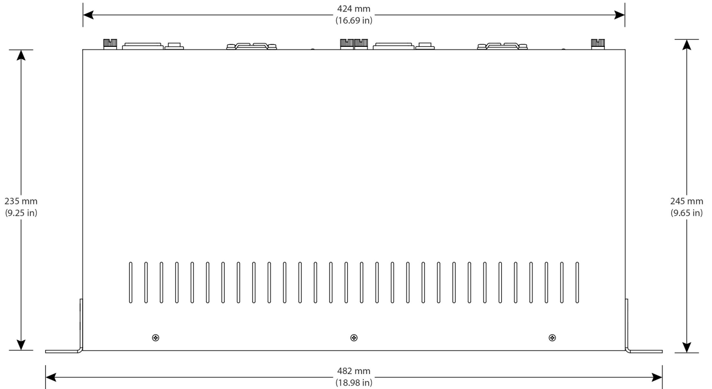
Top View with Rack Ears Installed
