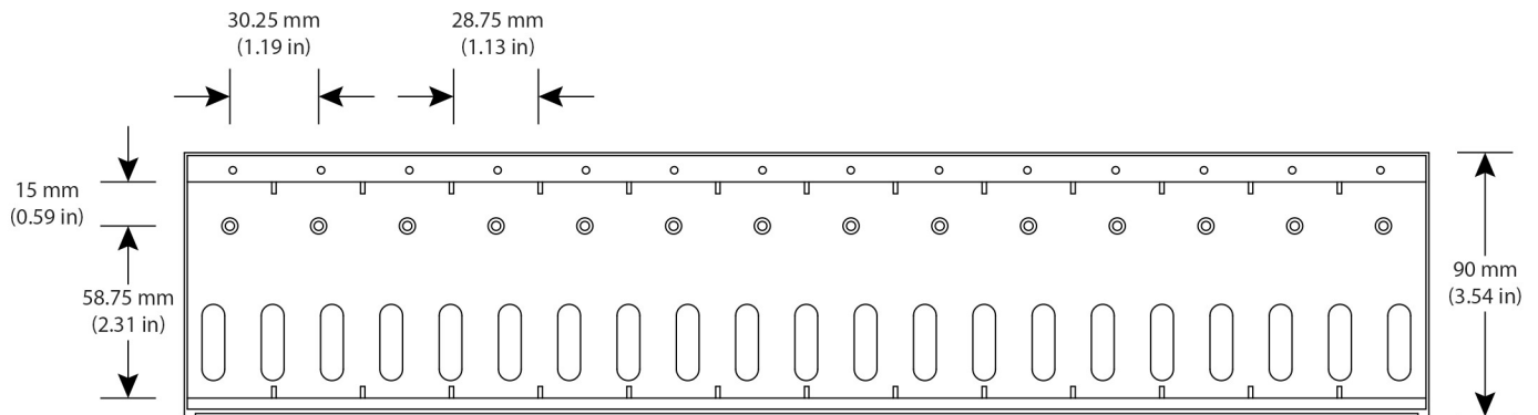
Front View with Rack Ears and Port Covers Removed
