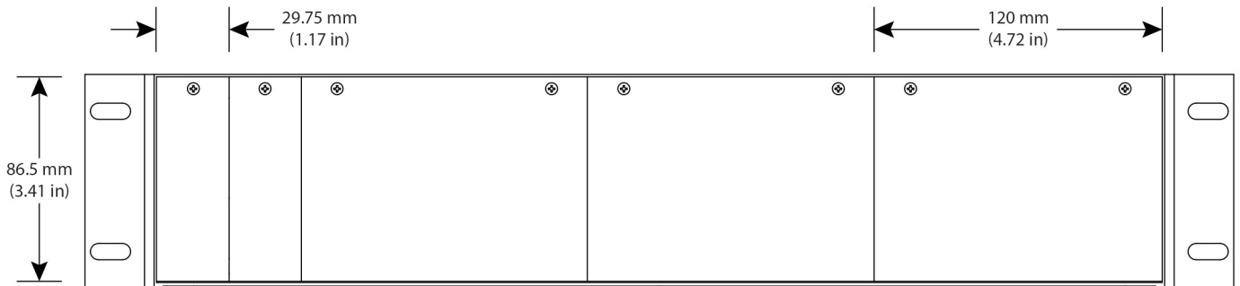
Front View with Rack Ears and Port Covers Installed
