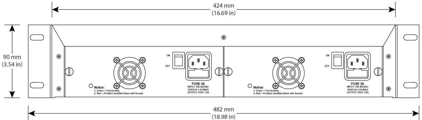
Rear View with Rack Ears Installed
