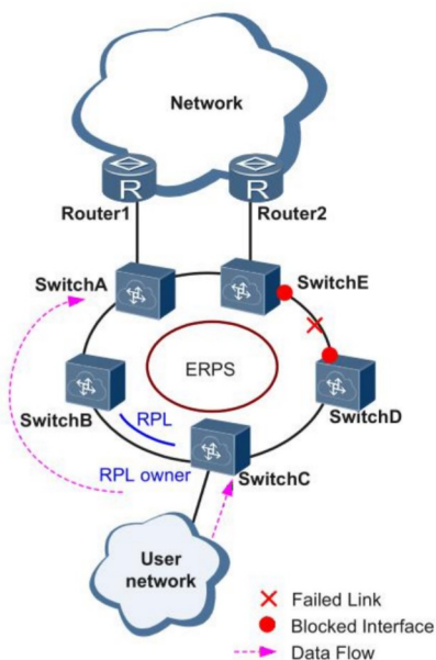
Figure 3-15 ERPS link failure
