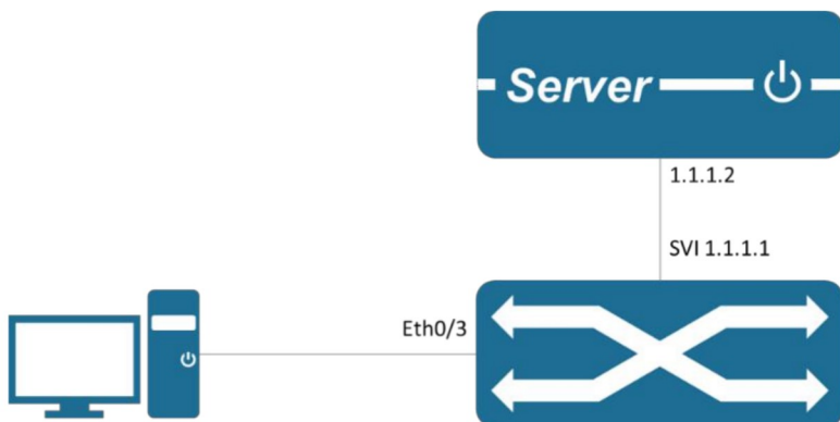
Figure 4-41 Typical MAC Authentication Networking Diagram
