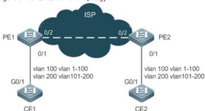
Figure 3-138 QinQ Network Topology 2
