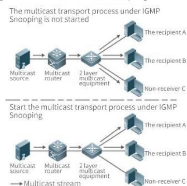
Figure 3-83 how IGMP Snooping works
