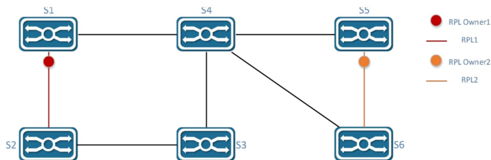
FIG. 3-17 ERPS tangential ring model
