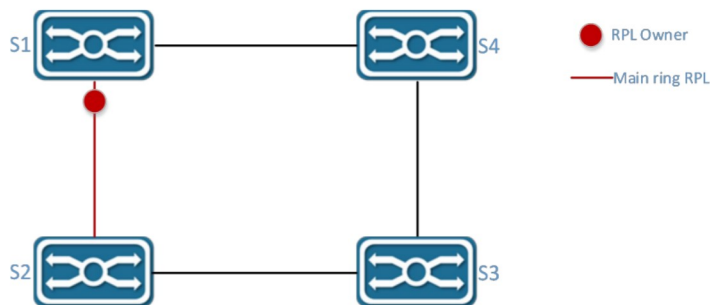
Figure 3-16 ERPS single-loop model
