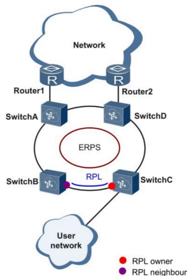
Figure 3-13 typical ERPS networking
