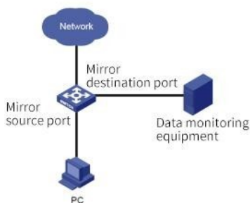
Figure 2-10 port mirroring
