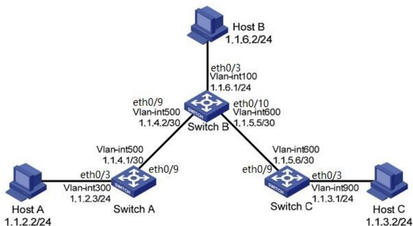
Figure 6-4 static routing configuration network diagram
