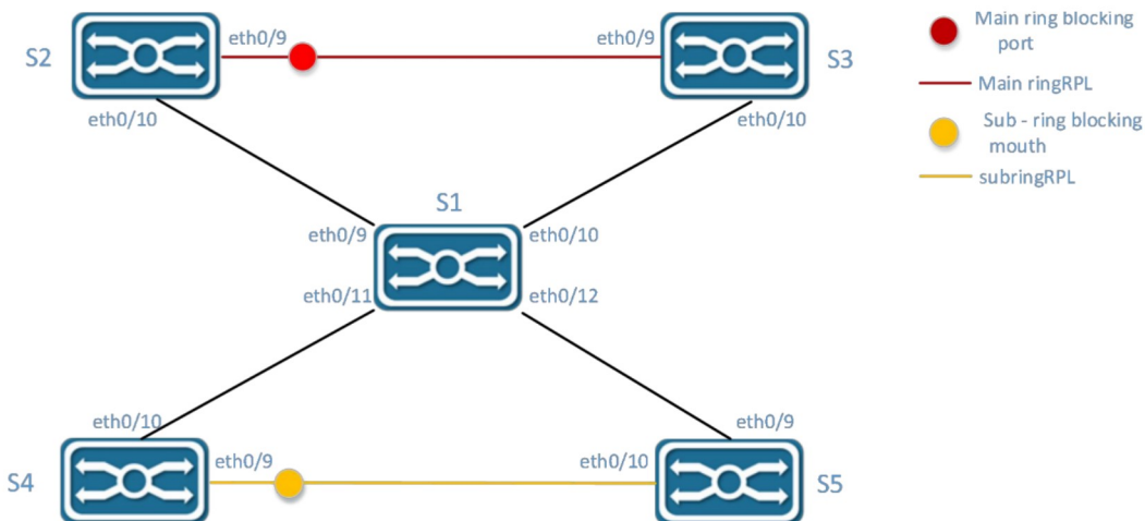
Figure 3-33 network topology
