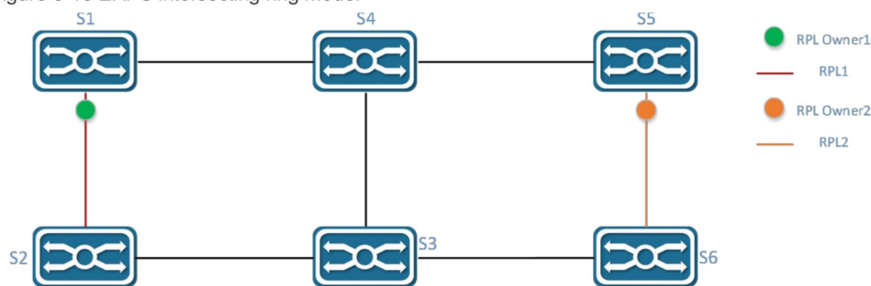
Figure 3-18 ERPS intersecting ring model
