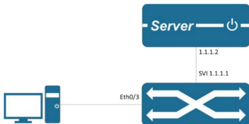
Figure 4-32 802.1X Authentication Typical Network Diagram
