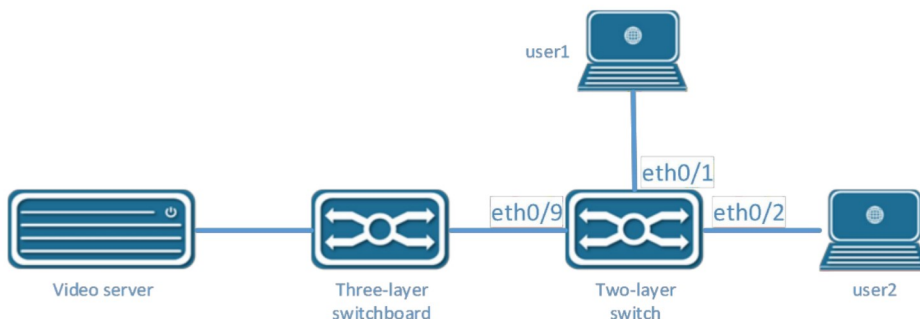
Figure 3-89 IGMP network topology
