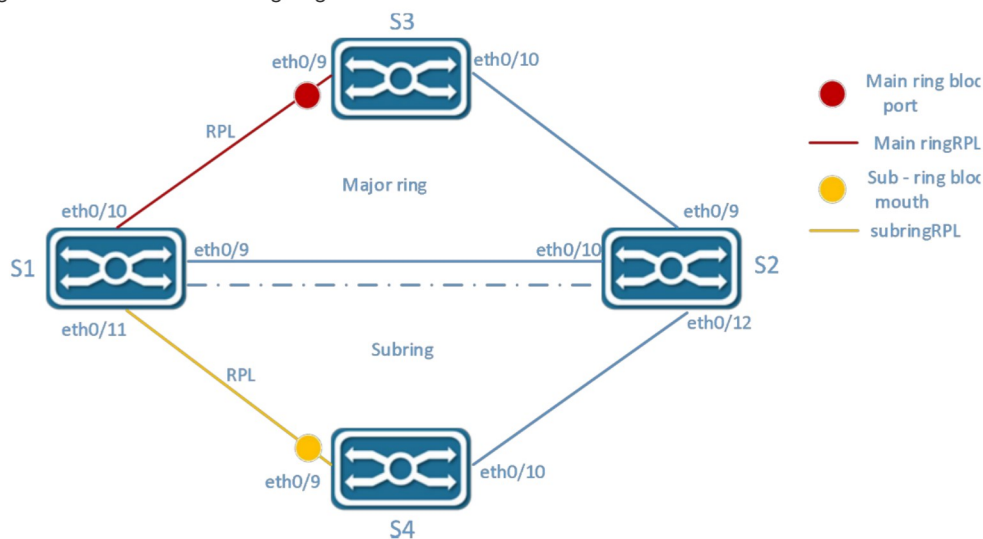
Figure 3-60 ERPS intersecting ring
