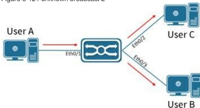
Figure 3-121 unknown broadcast 2
