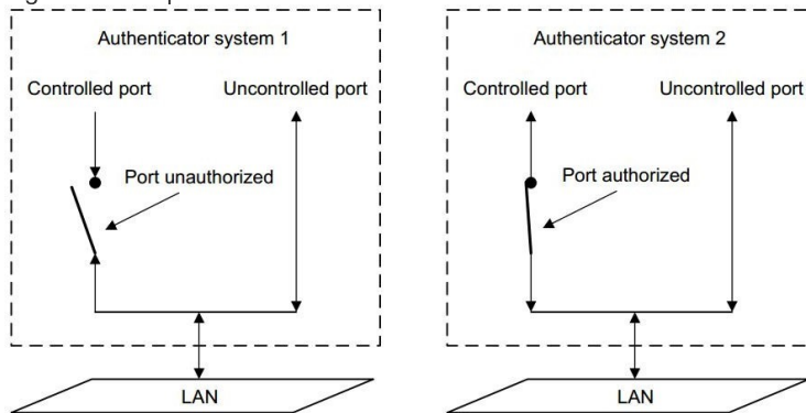
Figure 4-27 Impact of Authorization Status on Controlled Ports
