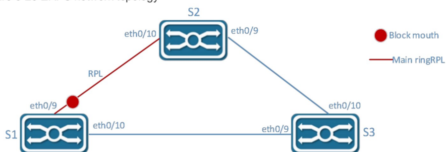
Figure 3-23 ERPS network topology
