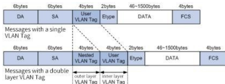
FIG. 3-127 QinQ's Packet Structure
