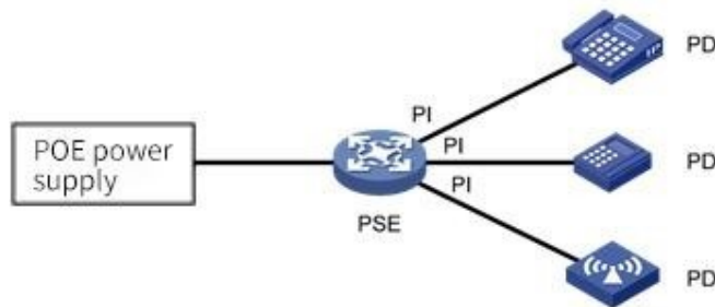
Figure 2-27 PoE system
