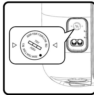
3. Adjust tap selector (if applicable)
