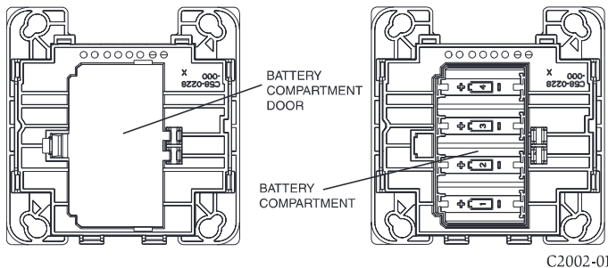
FIGURE 3. BATTERY COMPARTMENT:
