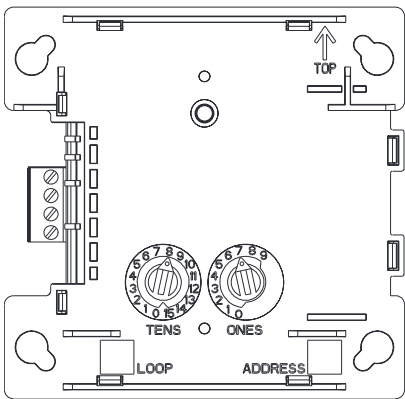
FIGURE 2. FACEPLATE INTERIOR:
