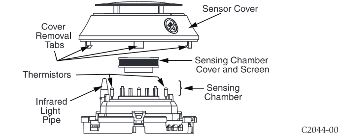
FIGURE 4. CLEANING THE PTIR DETECTOR
