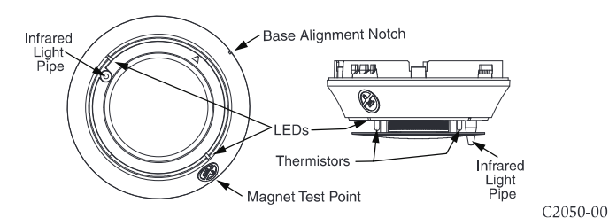
FIGURE 4. CLEANING THE PTIR DETECTOR
