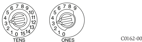
FIGURE 7. ROTARY ADDRESS SWITCHES
