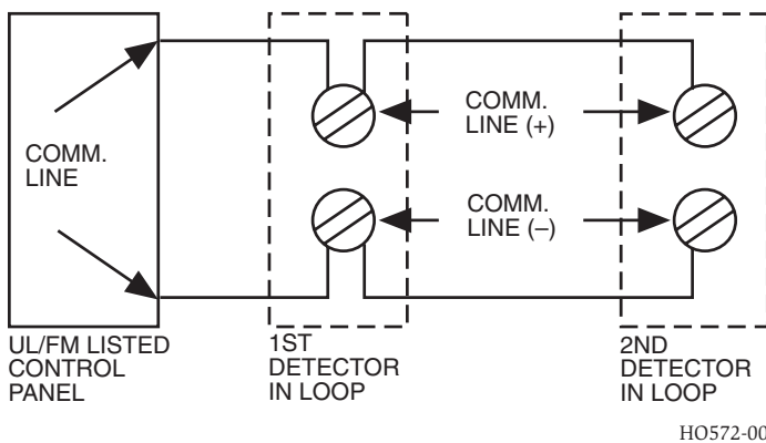
FIGURE 6. SYSTEM WIRING DIAGRAM FOR SK-DUCT-W
