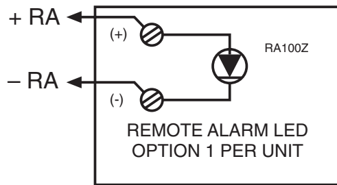
FIGURE 8. WIRING DIAGRAM FOR SK-DUCT-W TO RA100Z
