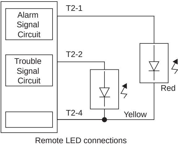
Figure 11-5: Wiring Diagram (Remote LEDs)
