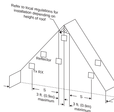
Figure 7-4: Sloped Ceiling (Peaked Type)
