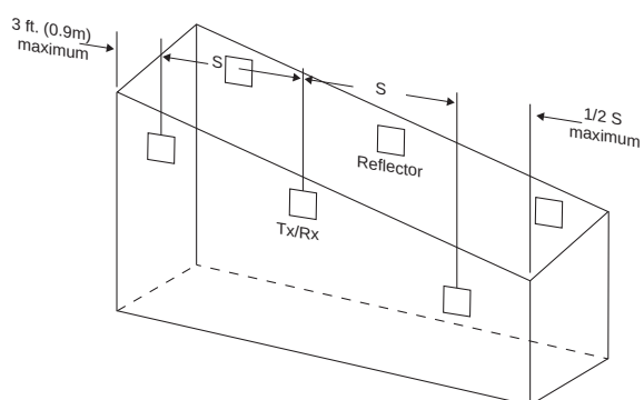
Figure 7-3: Sloped Ceiling (Shed Type)
