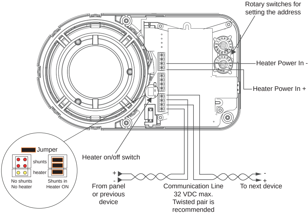
Figure 11-3: Wiring Diagram
