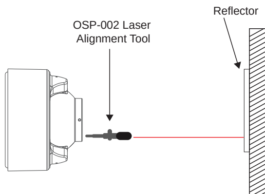
Figure 12-1: Coarse Alignment
