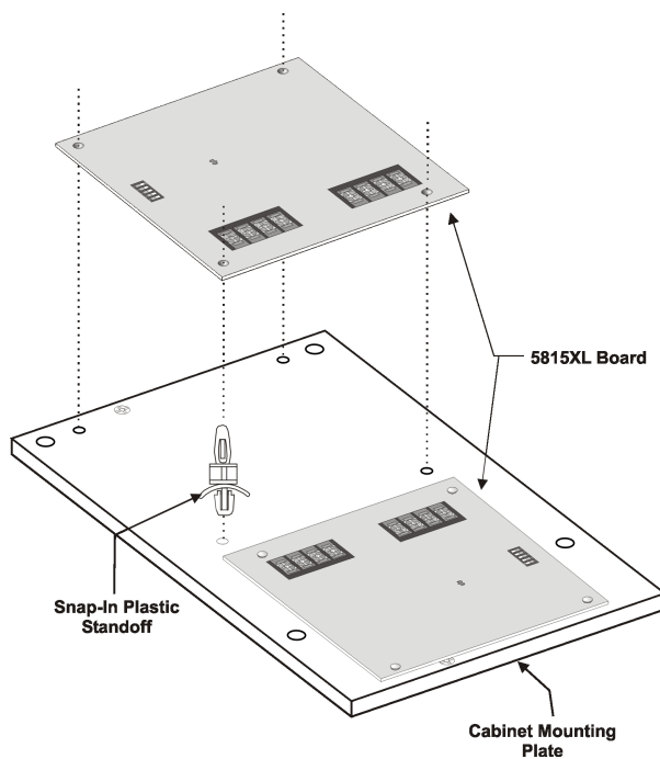
Figure 3: Standoff Installation
