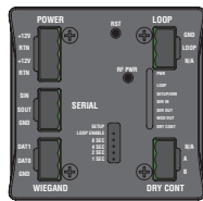
S2W-001 Wiegand Interface Module
