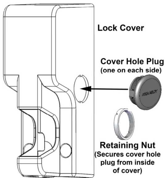
Figure 6. Cover Hole Plug and Retaining Nut
