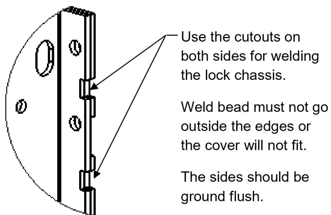
Figure 4. Chassis Welding
