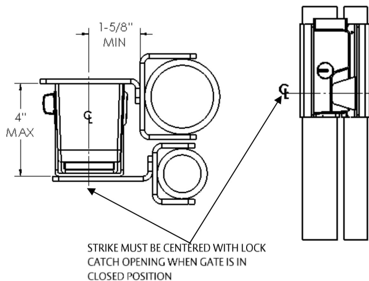
Figure 3. Installation Spacing Dimensions
