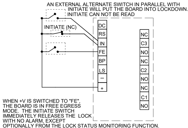
FIG. 4: OPTIONAL FREE EGRESS AND LOCKDOWN MODES
