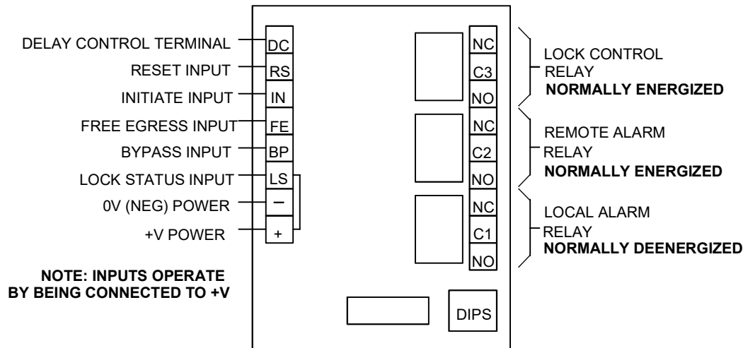
FIG. 1: OVERVIEW OF XDT BOARD
