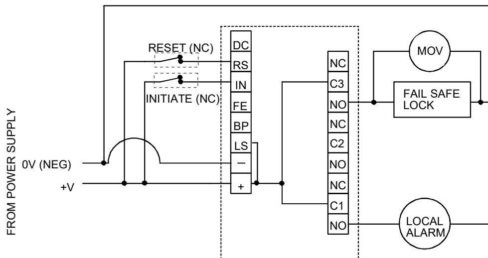
FIG. 2: TYPICAL XDT WIRING
