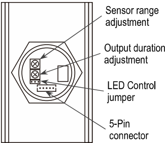
Sensor Back
