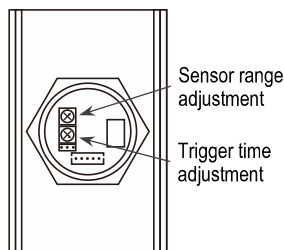
Fig. 2 Sensor Back
