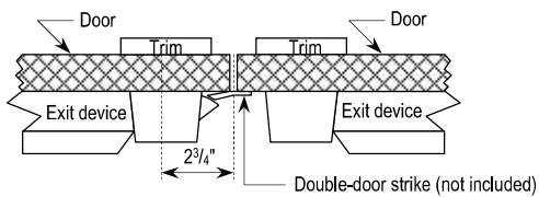
Double Door without Mullion
