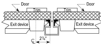
Double Door with Mullion
