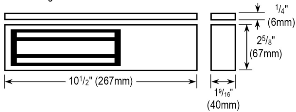
Electromagnet
