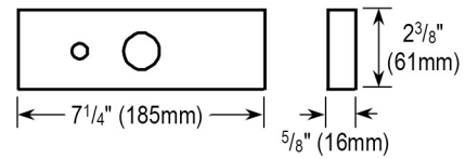
Armature Plate
