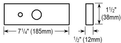
Armature Plate
