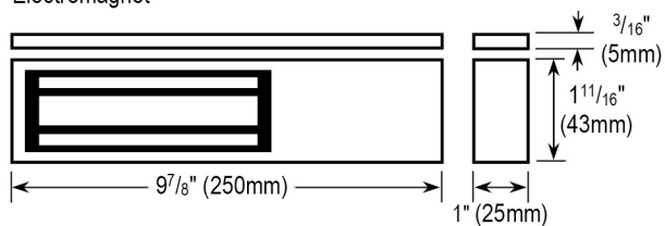
Electromagnet
