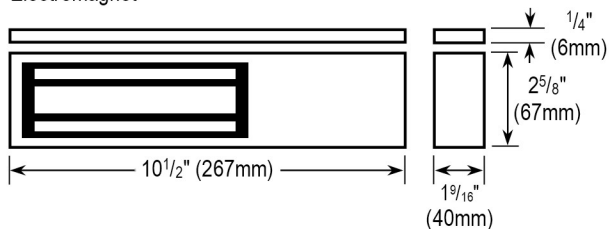
Electromagnet
