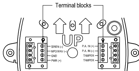
Fig. 3 Mounting base – terminal block detail
