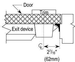
Double Door without Mullion
