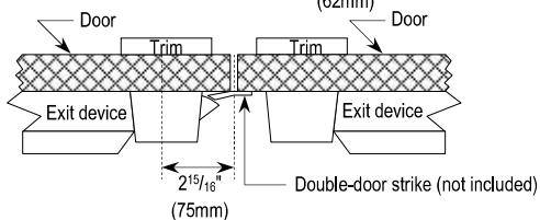
Double Door without Mullion
