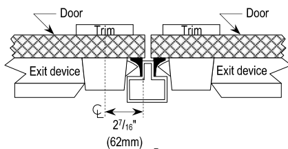
Double Door with Mullion
