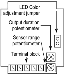
Fig.3 LED Jumper Settings
