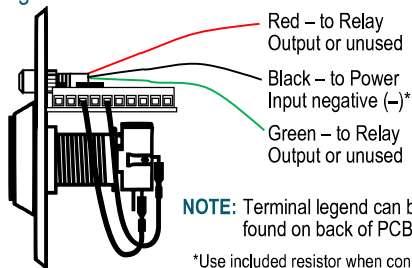
Fig. 9 – Side View
