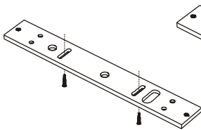
E-941Sx-600 mounting plate
