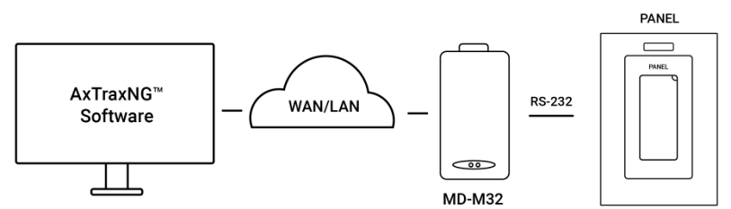
Figure 21: Connecting a Single Control Panel with MD-N32
