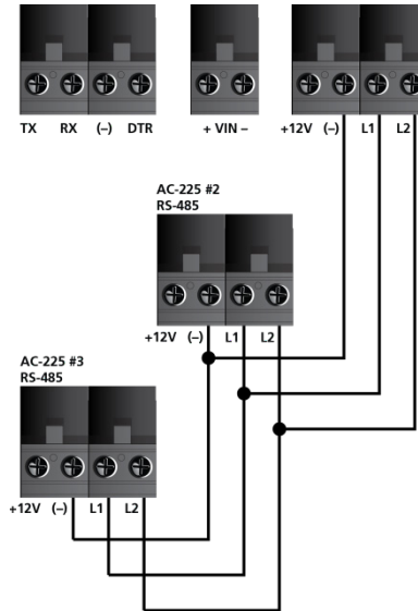
Figure 19: Daisy Chaining
