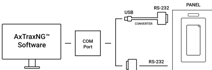
Figure 17: RS-232 Panel Connection to PC
