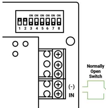
Figure 10: Normally Open Input Connection
