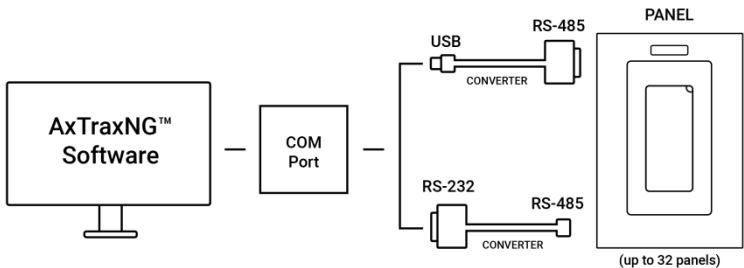
Figure 18: RS-485 Panel Connection to PC
