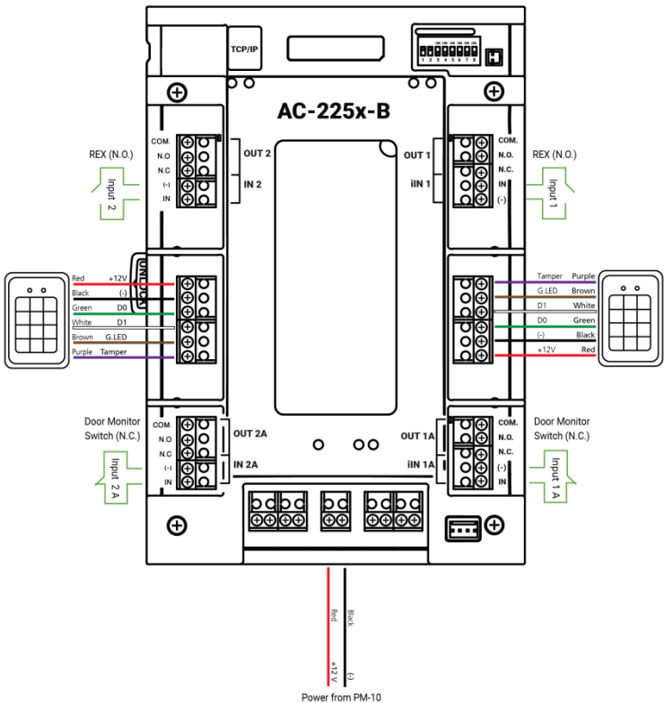
Figure 7: AC-225x-B Wiring Communications
