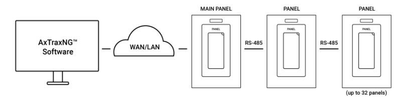
Figure 20: Connecting Multiple Access Control Panels to AC-225IP
