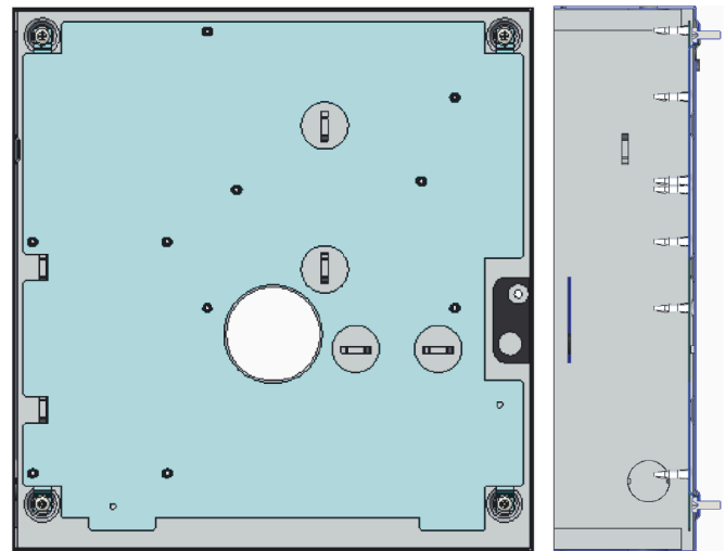
Figure 2: Installing the metal plate into a KT-300 (D31000201 rev 0/1)
