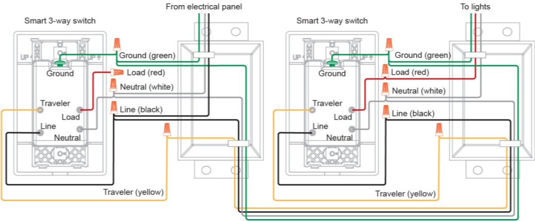
Figure 8: Connecting two IQ Power Switch-PG (3 way) to control one light from two places (3-way operation)
