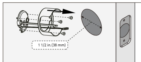
Figure 3: Exterior assembly hole dimension and removing the fire cup
