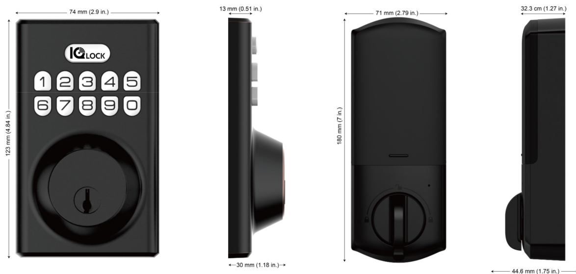
Figure 2: IQ Lock-PG dimensions
