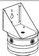
Wall mount option [BL-8400]
