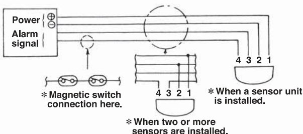
[Basic connection]
