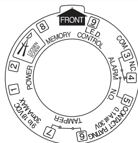
[Terminal arrangement-base]
