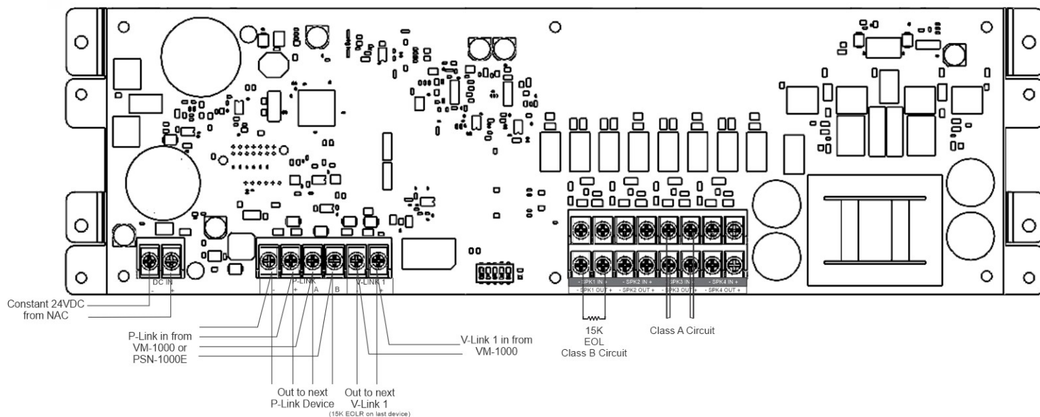
Fig 5 SCA-5070INT Connections
