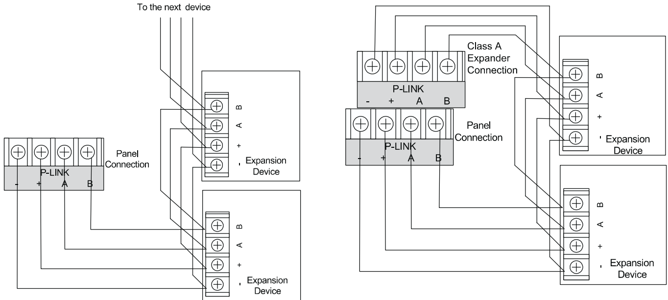
Figure 4. Examples of Wiring a RA-6500F as Class B and Class A
