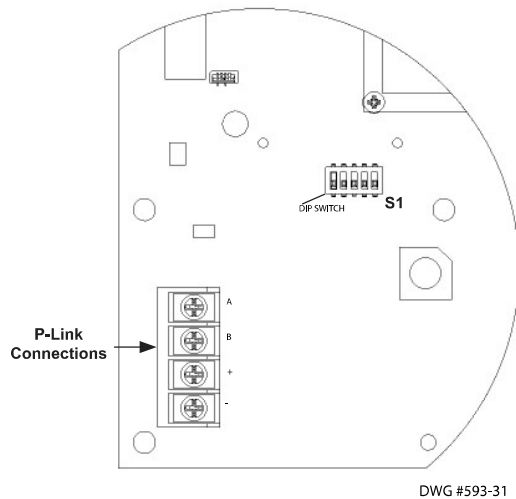
Figure 1. Example of Setting Address on the RA-6500F (panel view)
