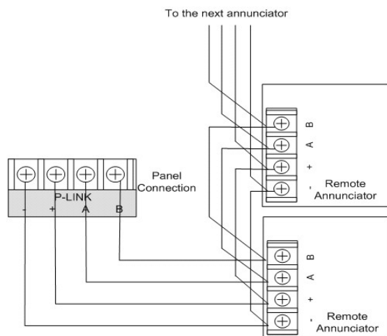
Figure 1: RA-6075 Class B Wiring Example
