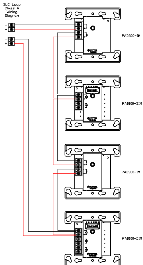
Figure 3. Example of Wiring a PAD300-IM as Class A
