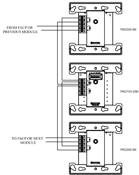
Figure 3. Example of Wiring a PAD300-IM as Class A
