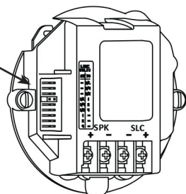
FIGURE 2: PAD100-SPKB Wiring and Power Tap
