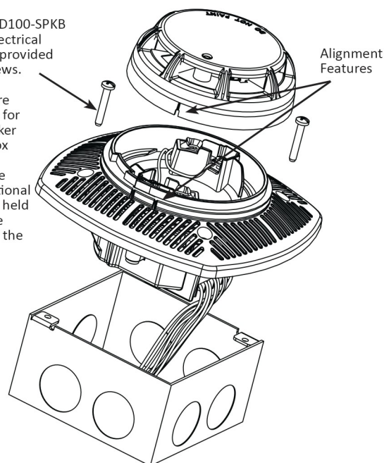
FIGURE 3a: Assembly of Detector on Electrical Box
