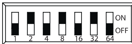
FIGURE 11: Enlarged View of PAD Device with Dip Switch Setting Addressed
