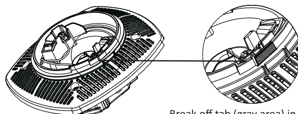
FIGURE 9: Disable Locking Feature
