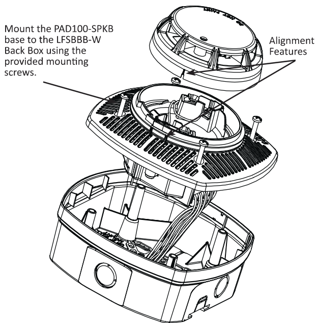
FIGURE 3b: Assembly of Detector on LFSBBB-W Back Box
