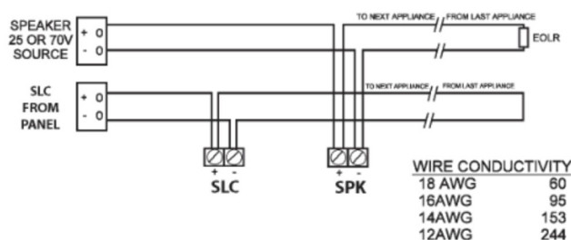
FIGURE 1: PAD100-SPKB Wiring Diagram
