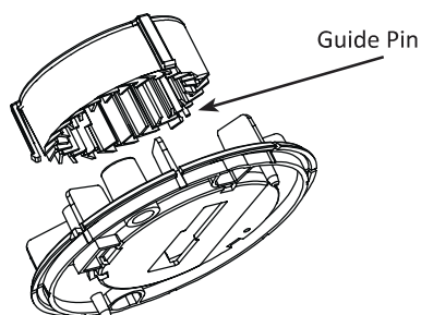
FIGURE 6: Replace Optic Cage into Optic Cage Base
