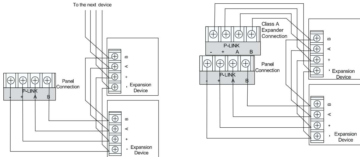
Figure 3. Examples of Wiring a PAD100-SLCE P-Link Class B & Class A Wiring
