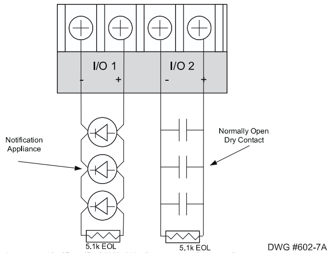
Figure 7. I/O Connections for Class A, Class X, or Class B. DWG #602-7A
