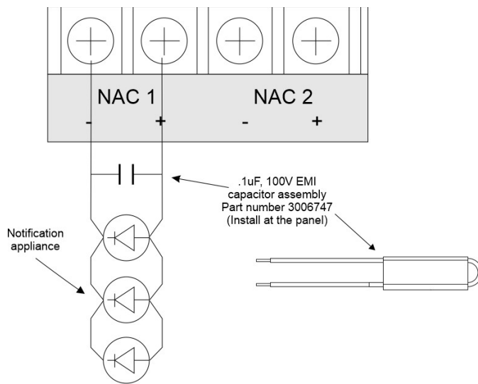
Figure 6. NAC EMI capacitor assembly wiring diagram
